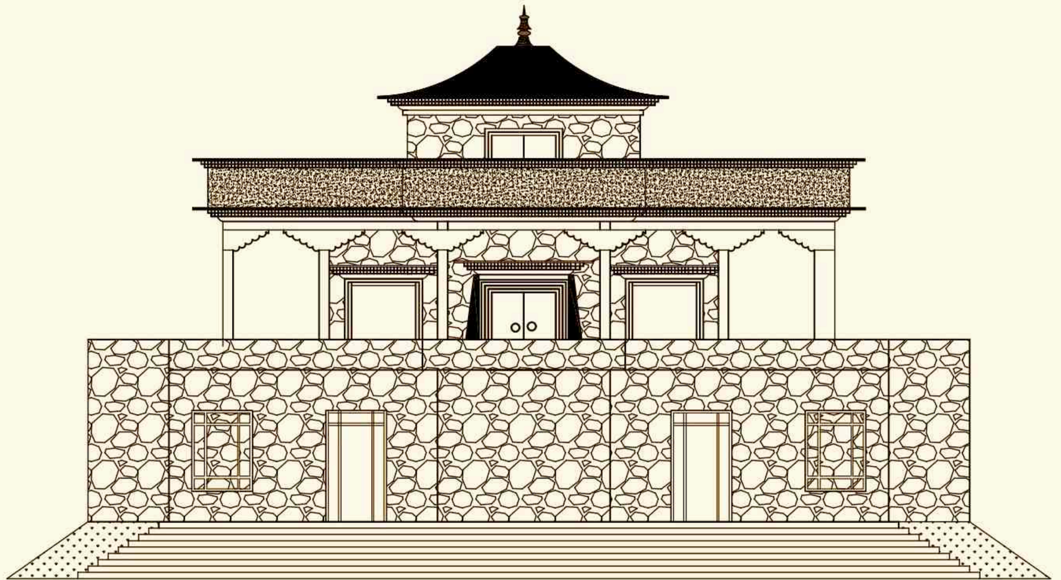
FRONT ELEVATION
